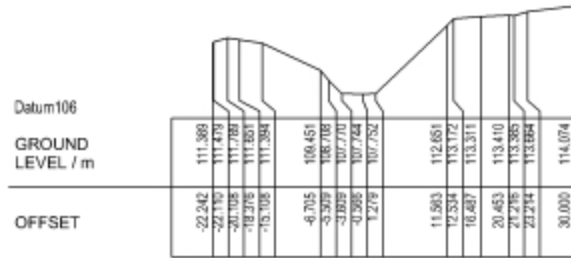
Cross Section 90.00
