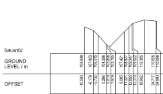
Cross Section 40.00
