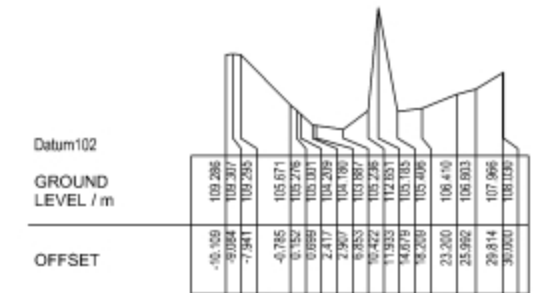
Cross Section 190.00
