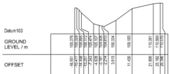
Cross Section 50.00
