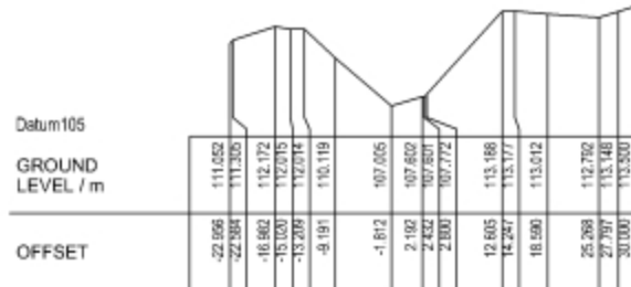
Cross Section 80.00
