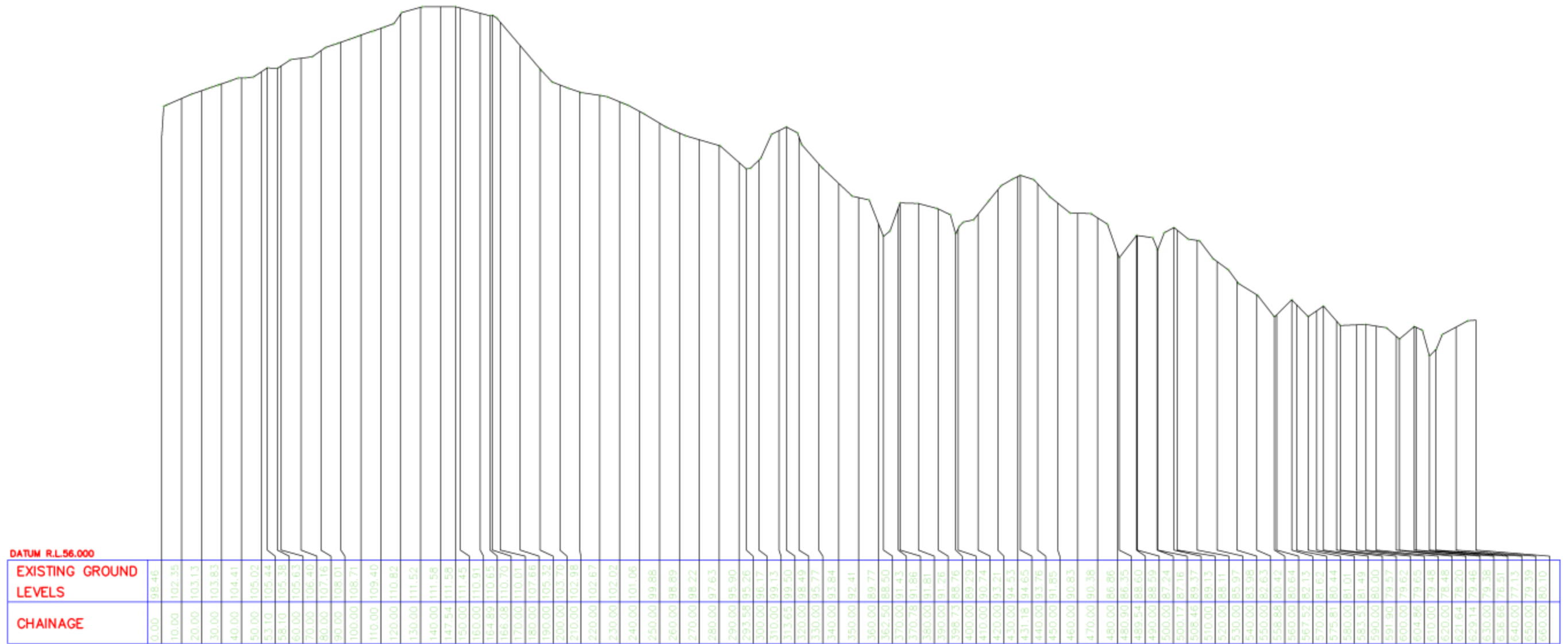
LONGITUDINAL SECTION – CROSS COUNTRY
